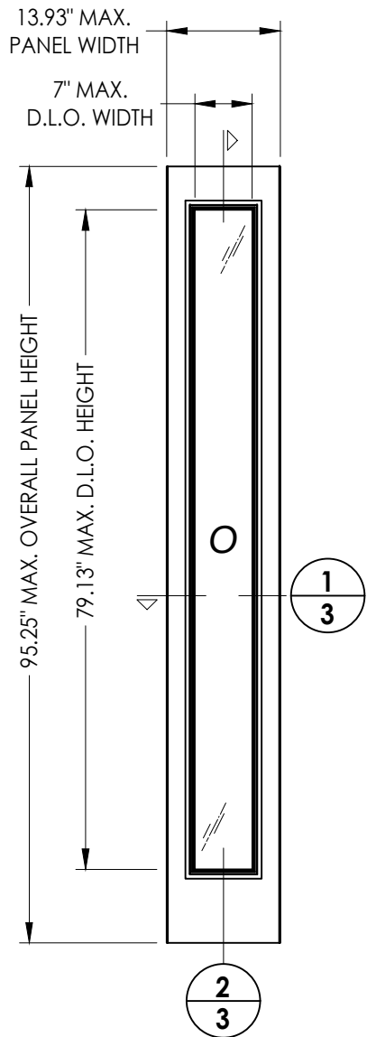
50 SIDELITE PANEL
