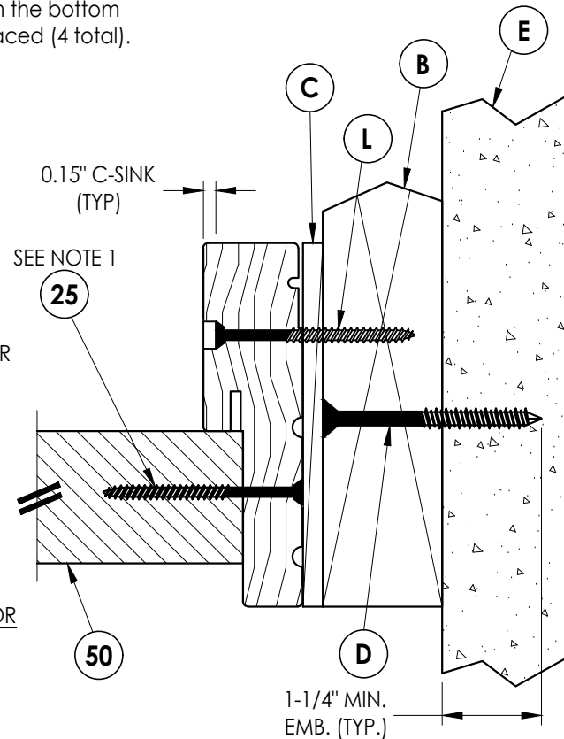
2 5 HORIZONTAL CROSS SECTION Outswing shown (Inswing similar)
