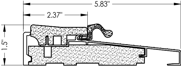
16 OUTSWING THRESHOLD
