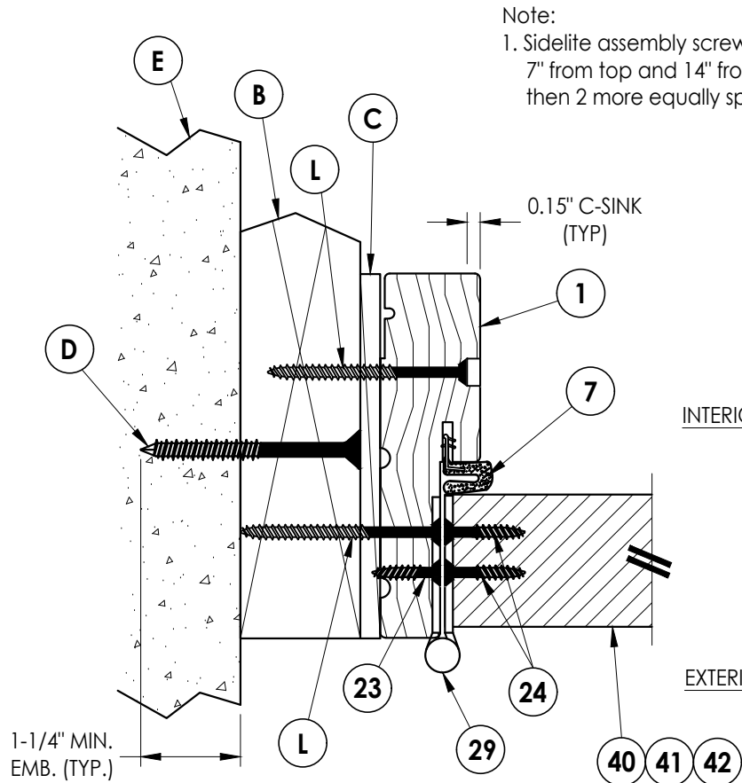
1 5 HORIZONTAL CROSS SECTION Outswing shown (Inswing similar)
