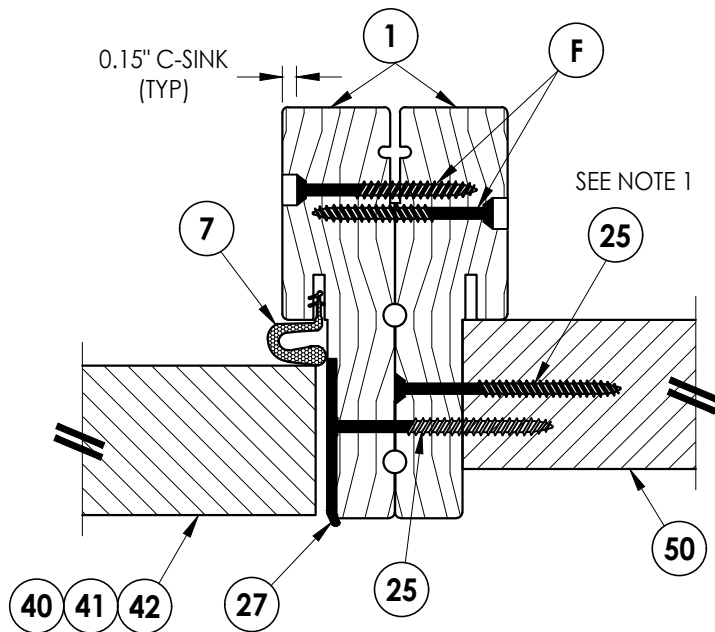
2 5 HORIZONTAL CROSS SECTION Outswing shown (Inswing similar)
